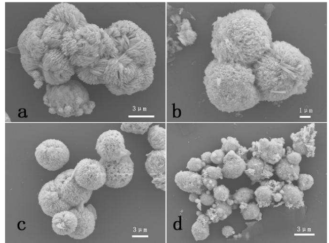
Figure 4. SEM images of the Tb_2(WO_4)_3 products with different surfactant (a) PVP, (b) Gly, (c) CTAB, (d) SDBS.
