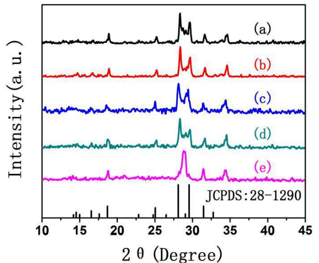
Figure 2. XRD patterns of Tb_2(WO_4)_3 products prepared using different surfactants (a) PVP, (b) Gly, (c) CTAB, (d) SDBS, (e) EDTA.
