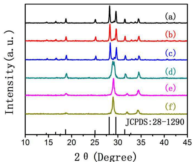
Figure 3. XRD patterns of Tb_2(WO_4)_3 products prepared using CTAB as surfactant at different pH values (a) 3, (b) 4, (c) 5, (d) 6, (e) 7, (f) 8.
