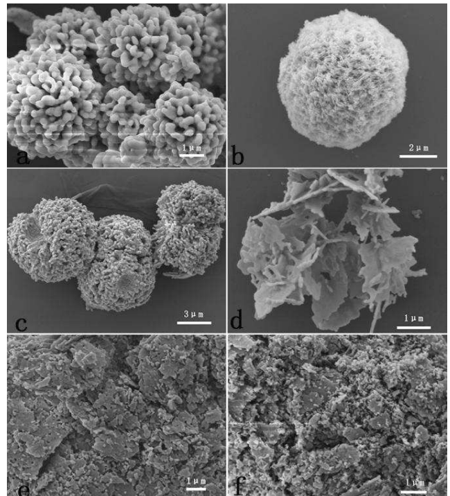
Figure 5. SEM images of Tb_2(WO_4)_3 products prepared using CTAB as surfactant at different pH values (a) 3, (b) 4, (c) 5, (d) 6, (e) 7, (f) 8.
